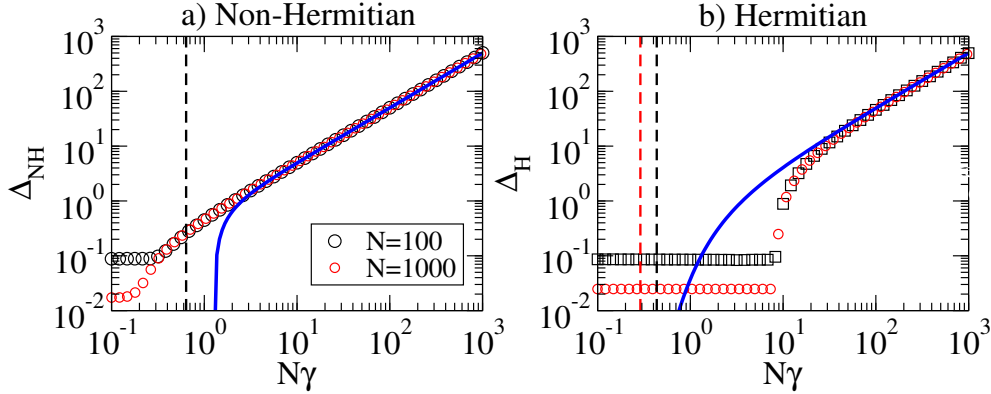
Figure 4.3: a) Gap \Delta_{NH} , vs. the coupling parameter N\gamma . Symbols are given by (4.9)-(4.10), while the continuous blue curve shows the analytical estimate (3.32) using S = 2\Omega . The dashed vertical line marks the critical coupling strength \gamma_{cr}^{NH} from Eq. (3.34). b) Gap \Delta_H , vs. the coupling parameter N\gamma . Symbols are given by (4.11) while the continuous blue curve shows the analytical estimate (3.17) using S = 2\Omega . The dashed vertical lines indicate the critical coupling strength \gamma_{cr}^H from Eq. (3.20). Here, W = 1 , N = \{100, 1000\} and the number of disorder configurations is N_r = 100 .
