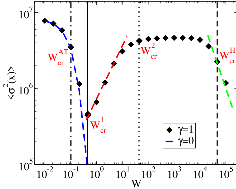
Figure 4.5: Average variance \langle \sigma^2(x) \rangle , see section 4.3.2, vs. disorder strength W for the coupling strength \gamma = 1 and the system size N = 10000 . Here, \Omega = 1 , \nu = 0 , N_r \times N = 10^5 where N_r is the number of disorder configurations. The vertical lines mark the critical disorders strength W_{\text{cr}}^{\text{AT}} , W_{\text{cr}}^1 , W_{\text{cr}}^2 or W_{\text{cr}}^{\text{H}} , see the description in section 4.4.2. The dashed blue curve shows the results for the Anderson model without long range hopping, \gamma = 0 . The dashed red line goes like W^{0.7} and the dashed green line goes like W^{-1} .
