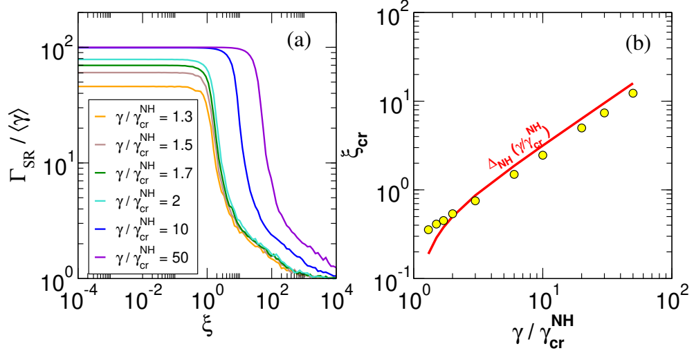
Figure 3.5: (a) Width of the superradiant state divided by the average width \langle \gamma \rangle = \gamma/N vs. the disorder strength \xi as introduced in the Hamiltonian (3.37)–(3.45)–(3.46). (b) The critical value \xi_{\text{cr}} (see text) is plotted vs. \gamma/\gamma_{\text{cr}}^{\text{NH}} as circles. The red line is the energy gap, as defined in Eq. (3.32). Parameters in both panels are N = 100 , S = 1 and an average over 100 realizations of static disorder is performed.
