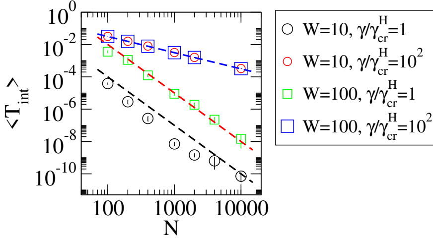
Figure D.1: Average integrated transmission \langle T_{\text{int}} \rangle vs. the system size N for the ground state, the normalized couplings strength \gamma/\gamma_{\text{cr}}^H = \{1, 100\} and the disorders strength W = \{10, 100\} . Here, \Omega = \nu = 1 , the number of disorder configurations N_r is such that N_r \times N = 10^5 . The dashed black and red lines are W^2/N^3 and the dashed blue line indicates the Eq. (D.1).
