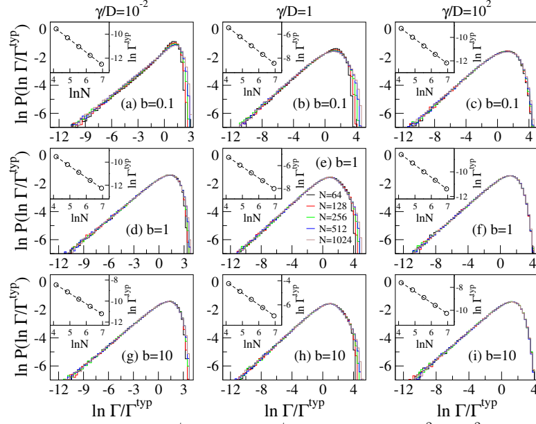
Figure 2.27: Distribution \ln P(\ln \Gamma / \Gamma^{\text{typ}}) vs. \ln \Gamma / \Gamma^{\text{typ}} for \gamma/D = \{10^{-2}, 1, 10^2\} and b = \{0.1, 1, 10\} for the scattering setup A. In the insets the scaling \Gamma^{\text{typ}} \propto N^{-\nu} is shown together with a linear fitting. Here, \Gamma^{\text{typ}} \equiv \exp \langle \ln \Gamma \rangle .
