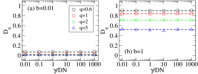
Figure 2.18: Multifractal dimensions D_q , q = \{0.6, 1, 2, 5\} , vs. the normalized coupling strength \gamma/DN for b = \{0.01, 1\} for the subradiant states. The dashed lines indicate the D_q of the closed PBRM model.
