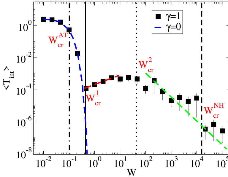
Figure 4.14: Average integrated transmission \langle T_{\text{int}} \rangle vs. the disorder strength W for the coupling strength \gamma = 1 and the system size N = 10000 for all the states. Here, \Omega = \nu = 1 , N_r \times N = 5 \times 10^5 where N_r is the number of disorder configurations. The vertical lines mark the critical disorders strength W_{\text{cr}}^{\text{AT}} , W_{\text{cr}}^1 , W_{\text{cr}}^2 or W_{\text{cr}}^{\text{H}} , see the description in section 4.4.2. The dashed blue curve shows the results for the Anderson model without long range hopping, \gamma = 0 . The dashed red line goes like W^{0.6} and the dashed green line goes like W^{-1.5} .
