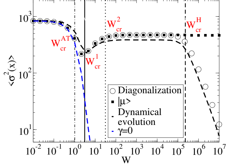
Figure 4.11: Average variance \sigma^2(x) vs. the disorder strength W for the coupling strength \gamma = 10^3 and the system size N = 100 . Here, N_r \times N = 10^5 where N_r is number of disorder configurations, the circles indicate the variance \sigma^2(x) obtained by diagonalize the total Hamiltonian H in Eq. (4.8), the squares are obtained by the perturbative approach in Eq. (4.39) and the dashed curves are the variance of the stationary distribution obtained by dynamical evolution of a localized excitation. The vertical lines mark the critical disorders strength W_{cr}^{AT} , W_{cr}^1 , W_{cr}^2 or W_{cr}^H , see the description in section 4.4.2. The dashed blue curve shows the results for the Anderson model without long range hopping, \gamma = 0 .
