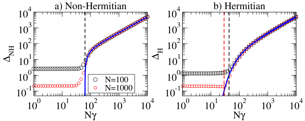
Figure 4.2: a) Gap \Delta_{\text{NH}} , vs. the coupling parameter N\gamma . Symbols are computed numerically using the expressions (4.9)-(4.10), while the continuous blue curve shows the analytical estimate (3.32). The dashed vertical line marks the critical coupling strength \gamma_{\text{cr}}^{\text{NH}} from Eq. (3.34). b) Gap \Delta_{\text{H}} , vs. the coupling parameter N\gamma . Symbols are given by (4.11) while the continuous blue curve shows the analytical estimate (3.17). The dashed vertical lines indicate the critical coupling strength \gamma_{\text{cr}}^{\text{H}} from Eq. (3.20). Here, W = 100 , N = \{100, 1000, 4000\} and the number of disorder configurations is N_r = 100 .
