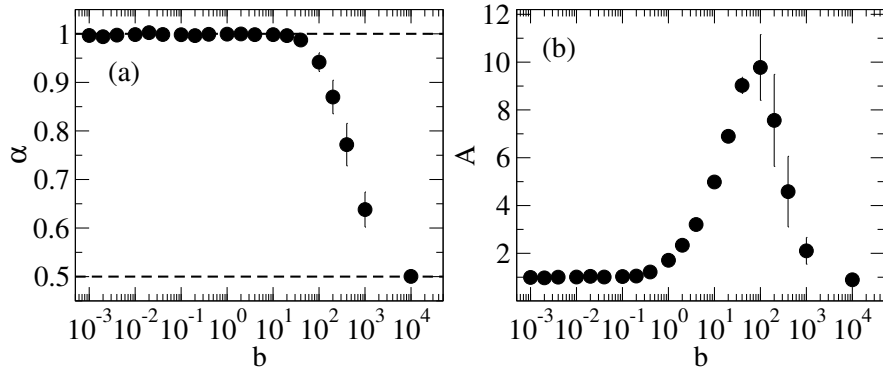
Figure 2.9: Fitting parameters (a) \alpha and (b) A as function of bandwidth b , from the fittings of the data on Figs. 2.7 and 2.8 with Eq. (2.25).
