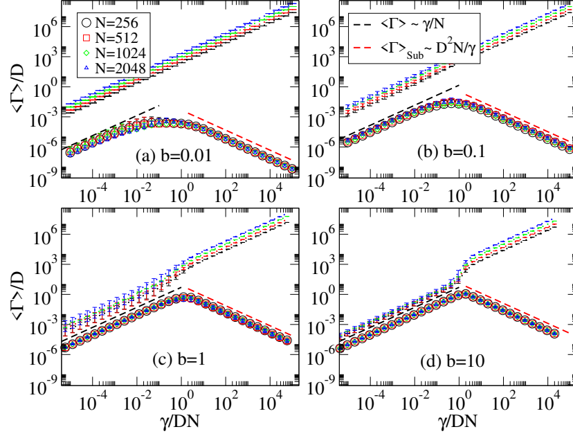
Figure 2.11: Same as in Fig. 2.10 for the scattering setup B with the coupling strength \gamma normalized by DN .
