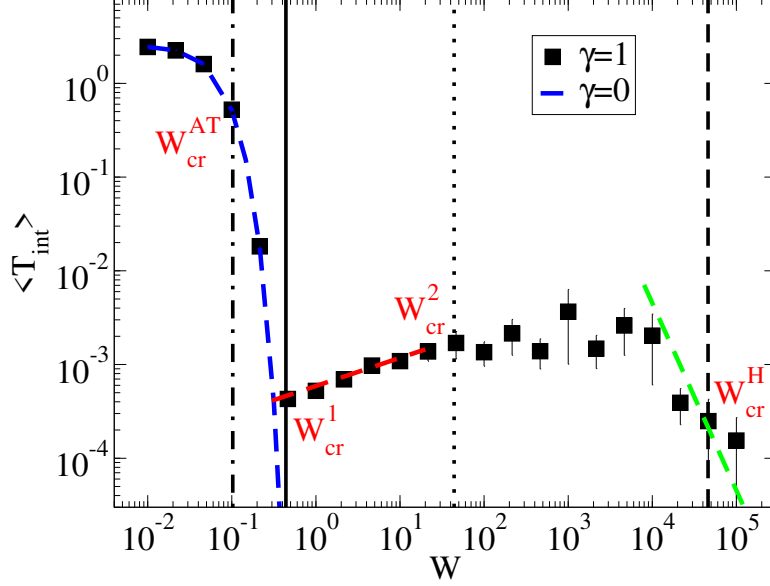
Figure 4.6: Average integrated transmission \langle T_{\text{int}} \rangle vs. the disorder strength W for the coupling strength \gamma = 1 and the system size N = 10000 . Here, \Omega = \nu = 1 , N_r \times N = 5 \times 10^5 where N_r is the number of disorder configurations. The vertical lines mark the critical disorders strength W_{\text{cr}}^{\text{AT}} , W_{\text{cr}}^1 , W_{\text{cr}}^2 or W_{\text{cr}}^H , see the description in section 4.4.2. The dashed blue curve shows the results for the Anderson model without long range hopping, \gamma = 0 . The dashed red line goes like W^{0.3} and the dashed green line goes like W^{-2} .
