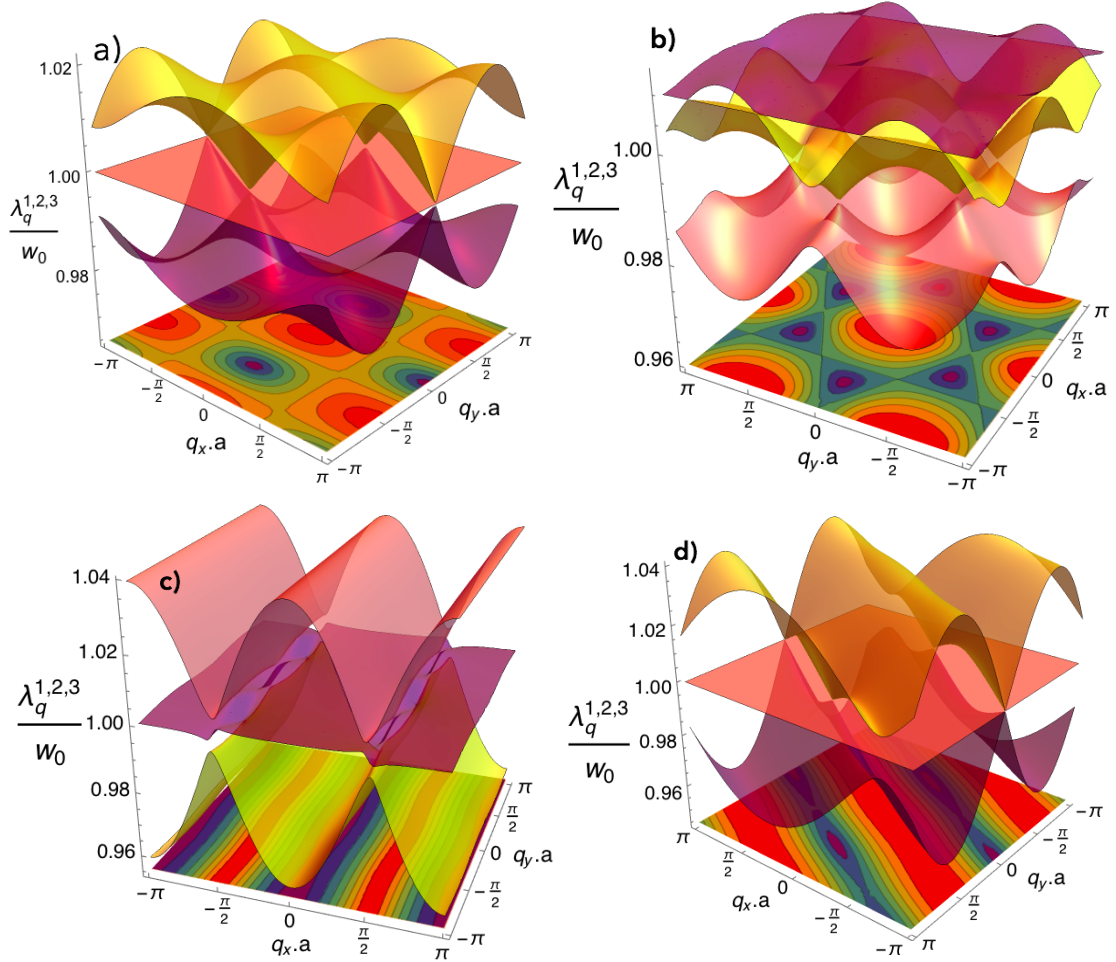
Figura 4.10: CPs para: \varphi = 90^\circ . a) \theta = \arcsen[1/\sqrt{3}] , C_0 = C_2 = 3/4 y C_1 = 0 . b) \theta = \pi/4 , C_0 = C_2 = 7/16 y C_1 = 1 . c) \theta = \pi/2 , C_0 = C_2 = 1/4 y C_1 = -2 . d) \varphi = \arccos[1/\sqrt{3}] + 90^\circ , y \theta = \pi/2 , C_{0,2} = 1 - 3\text{sen}^2(\pi/6 \pm \arccos(1/\sqrt{3})) y C_1 = 0 .
