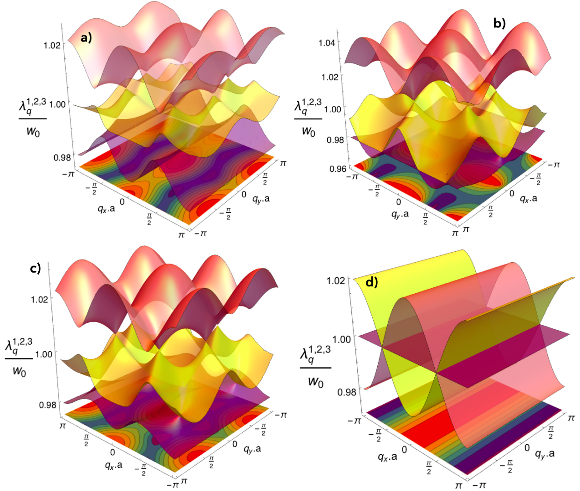
Figura 4.6: Dispersión colectiva de plasmones para: a) \theta = 30^\circ , C_1 = 1, C_2 = C_0 = \frac{7}{16} . b) \theta = \pi/2 , C_1 = 1, C_2 = C_0 = -\frac{5}{4} . c) \theta = 60^\circ , C_1 = 1, C_2 = C_0 = -11/16 . d) \theta = \arcsen[2/3] , C_1 = 1, C_2 = C_0 = 0 .
