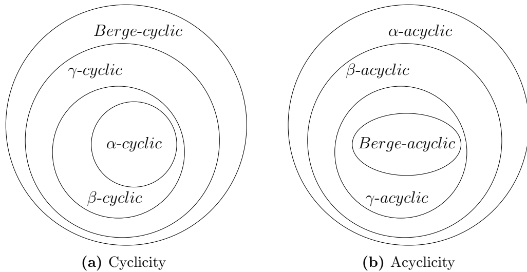
Figure 3.8: Cyclicity and acyclicity relationships on hypergraphs.
