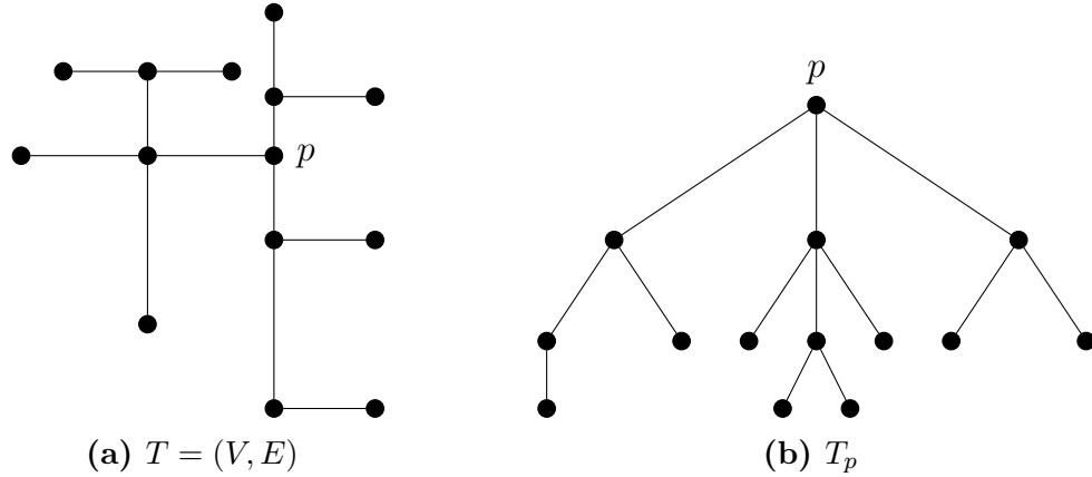
Figure 2.5: A tree rooted at a given vertex.
