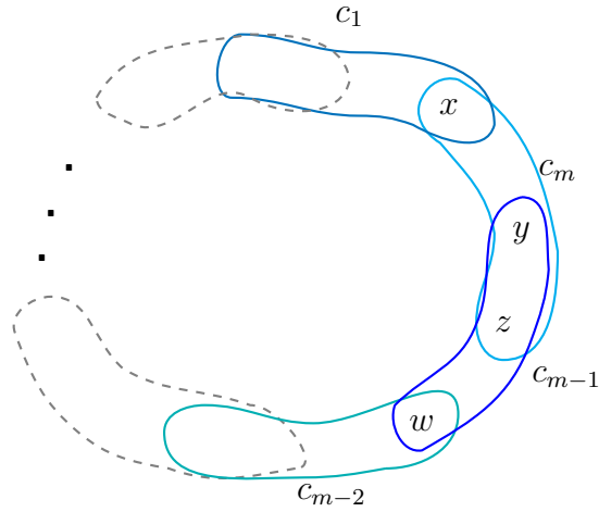
Figure 4.5: Alternating cycles, case 2 of theorem 4.4
