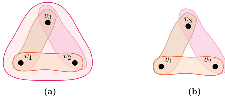
Figure 3.6: (a) \alpha -acyclic hypergraph H . (b) \alpha -cyclic hypergraph H' .
