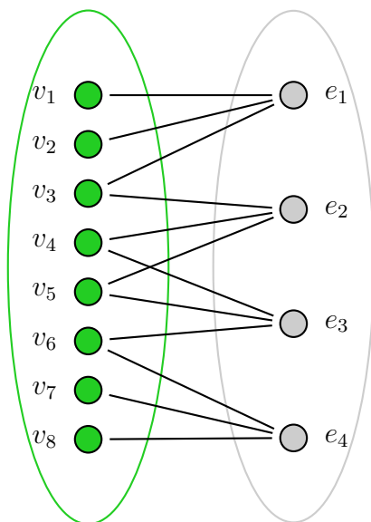
Figure 3.7: Incidence graph for hypergraph in figure 3.1 .
