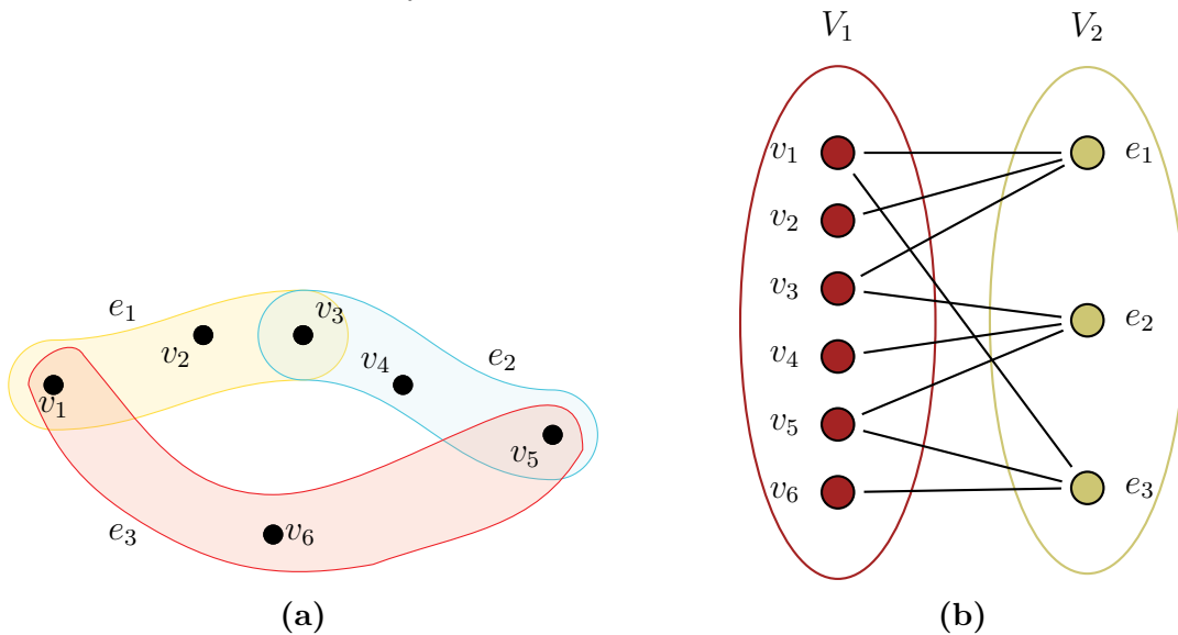
Figure 2.3: Hypergraph H (left) and its incidence graph (right).
