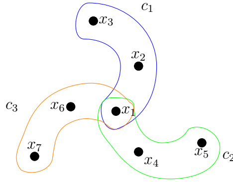
Figure 4.1: Hypergraph associated with \varphi = \{c_1, c_2, c_3\}
