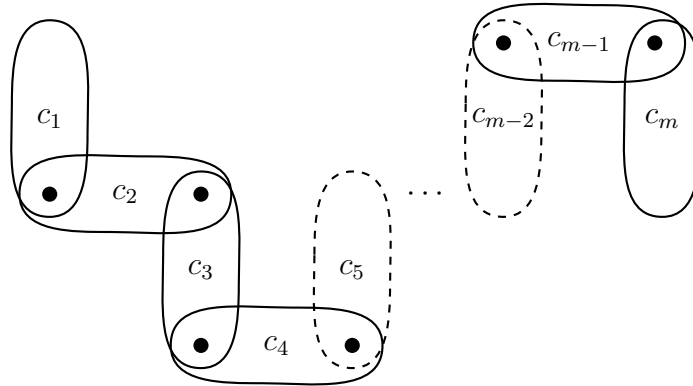
Figure 3.10: A simple chain \varphi .
