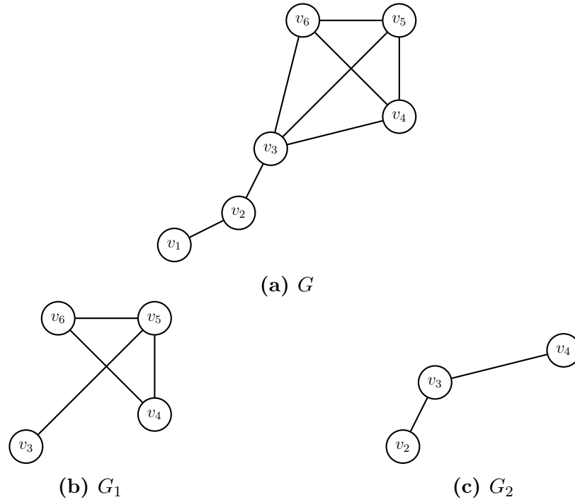
Figure 1.7: G_1 is a subgraph of G and G_2 is an induced subgraphs of G .
