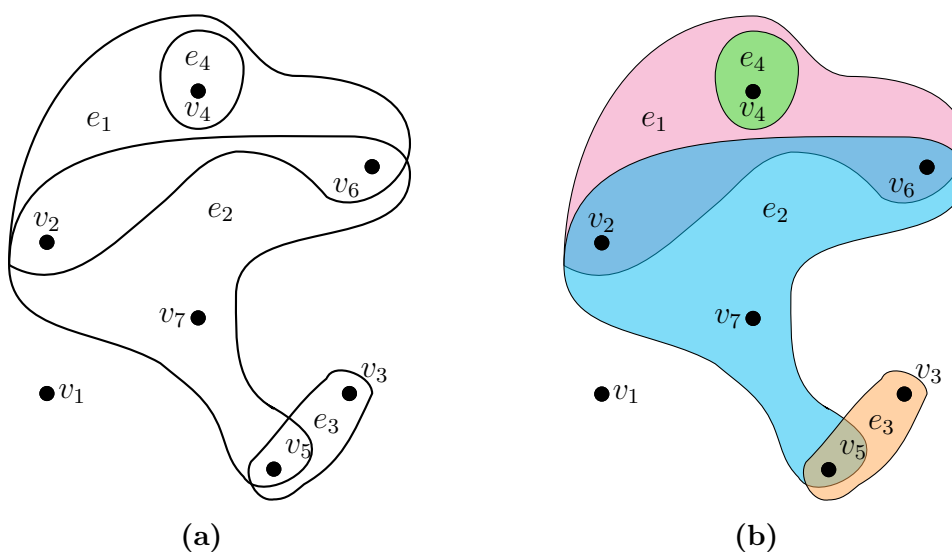
Figure 2.2: A hypergraph H .
