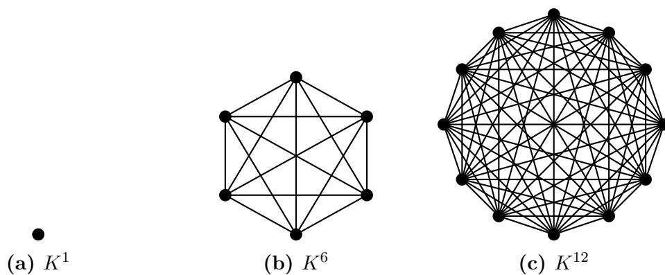
Figure 1.2: Complete graphs.
