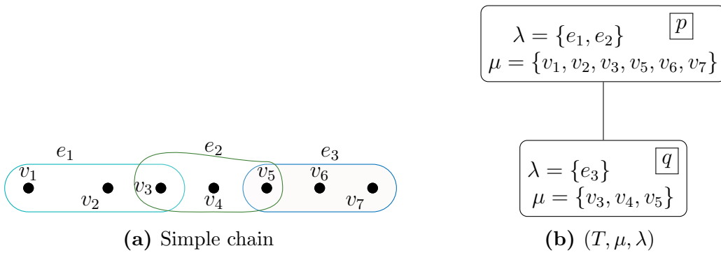
Figure 4.6: A simple chain and its tree decomposition of width 2.
