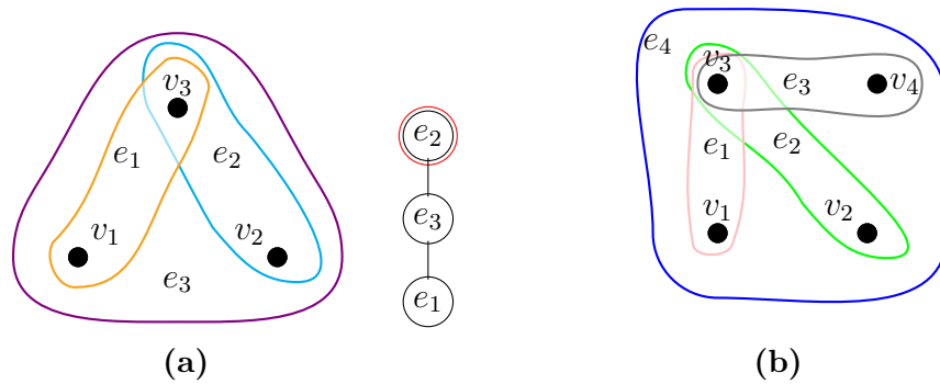
Figure 3.5: (a) A \gamma -cyclic hypergraph and its join tree with disjoint branches. (b) A \beta -acyclic hypergraph having no join tree with disjoint branches.
