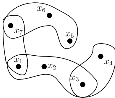
Figure 3.9: Associated hypergraph of the formula \varphi = (x_1 \vee x_2 \vee x_3) \wedge (x_3 \vee x_4) \wedge (x_5 \vee x_6 \vee x_7) \wedge (x_1 \vee x_7) .
