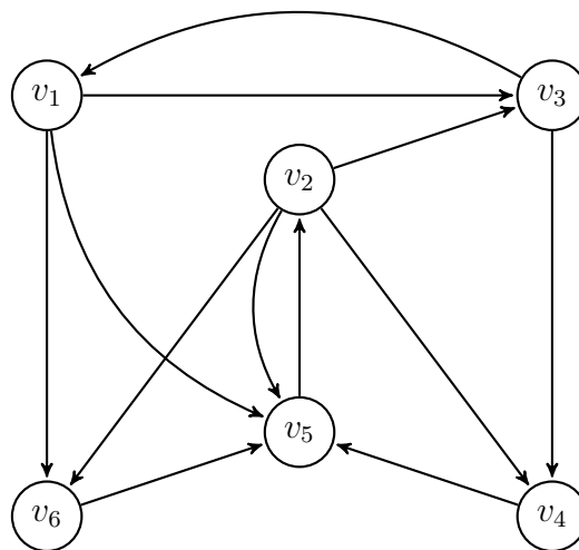
Figure 1.4: A digraph.
