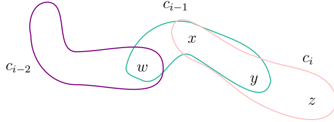
Figure 4.3: Alternating chain, case 2 of theorem 4.2
