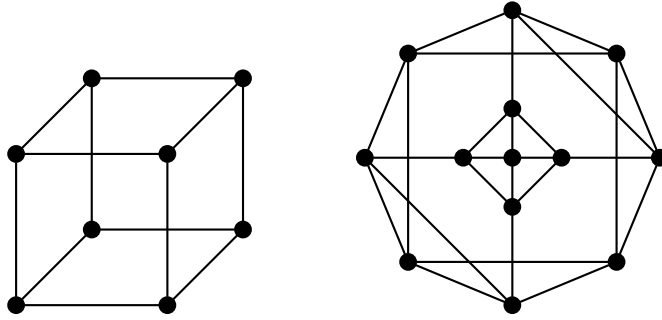
Figure 1.6: Regular graphs.
