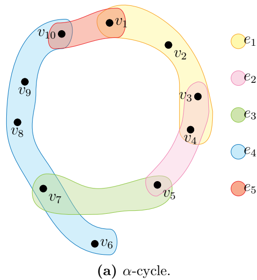
Figure 3.3: Three different degrees of cyclicity in hypergraphs.
