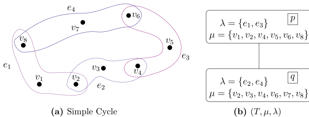
Figure 4.8: A simple cycle and its tree decomposition of width 2.
