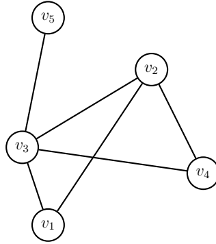
Figure 1.1: Simple graph G = (V, E) .
