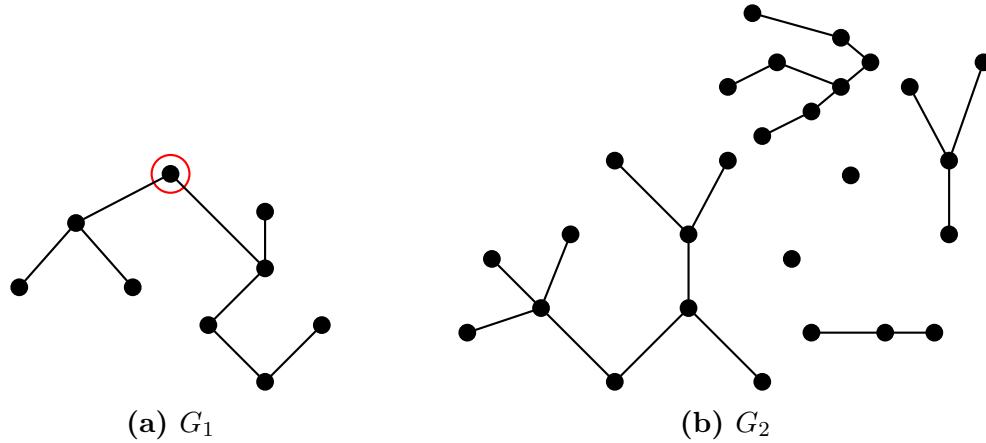
Figure 1.8: G_1 is a rooted tree and G_2 is a forest.
