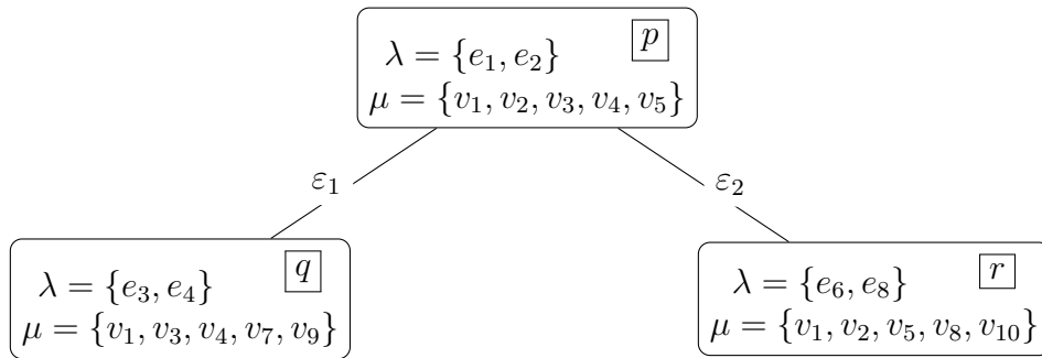
(b) (T, \mu, \lambda)
