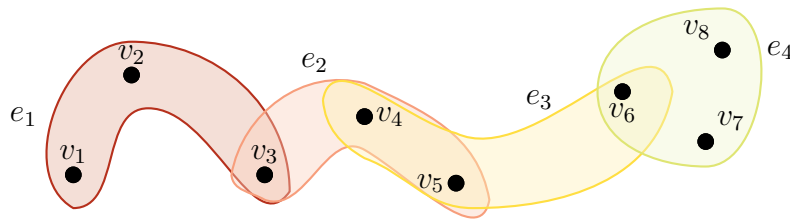
Figure 3.1: A Berge-cyclic hypergraph.
