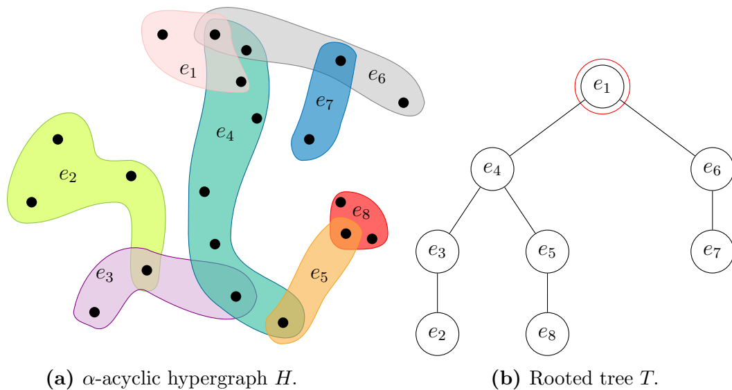
Figure 3.4: Join tree T of hypergraph H .
