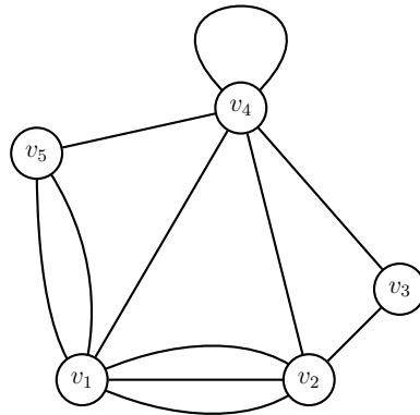
Figure 1.3: A multigraph G .
