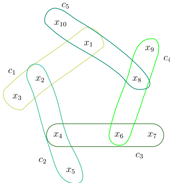
Figure 4.4: Simple cycle
