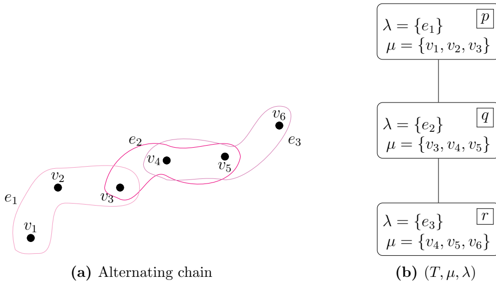
Figure 4.7: An alternating chain and its tree decomposition of width 1.
