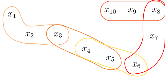
Figure 4.2: Alternating chain.
