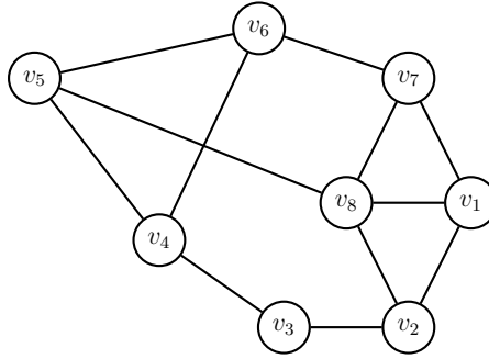
Figure 1.9: G = (V, E) .
