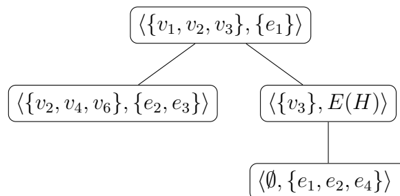
Figure 2.4: A hypertree for the hypergraph in figure 2.2
